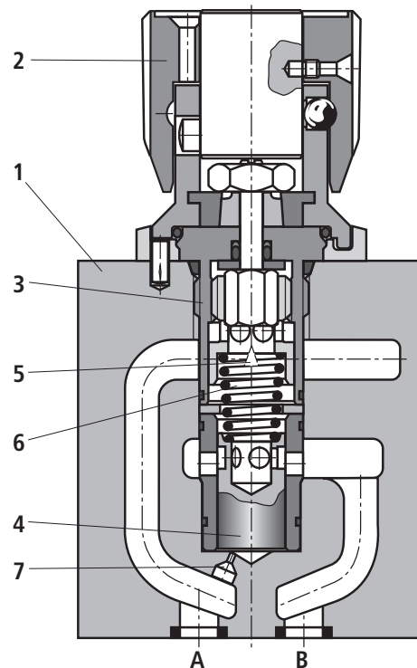
Type 2FRM 6 B76-3X/.M...
