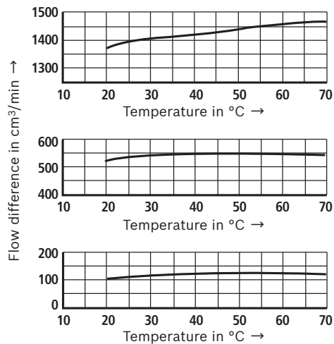
Temperature dependency at \Delta p = 20 \text{ bar}
