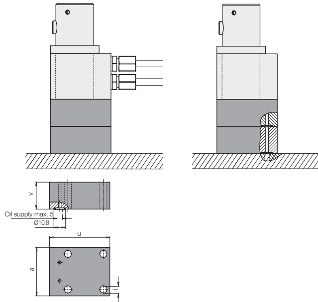
Part no. 0191-501
