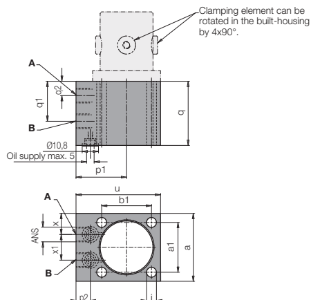
Part no. 0191-500
