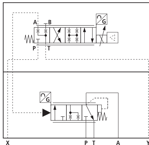
Pilot valve 4WRPEH6
