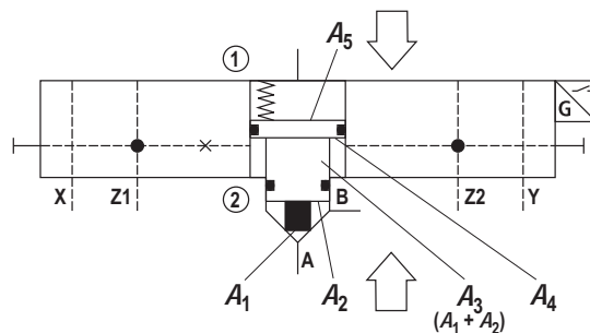
Type LC2A 025 ...-1X/.Q7G24... (with control cover type LFA . D... and monitoring of the closed position of the valve poppet)
