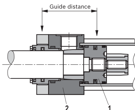
Without support width extension
