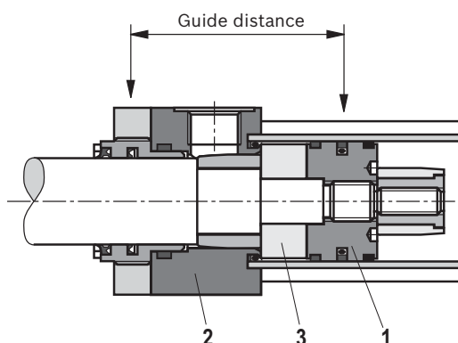
With support width extension
