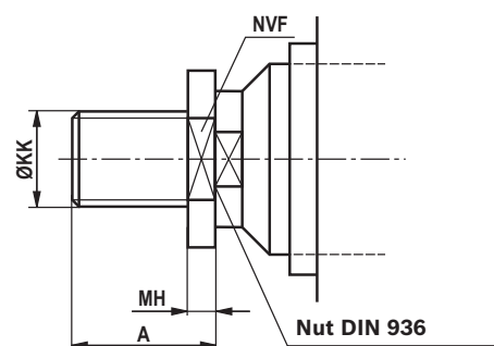
Piston rod end "F"
