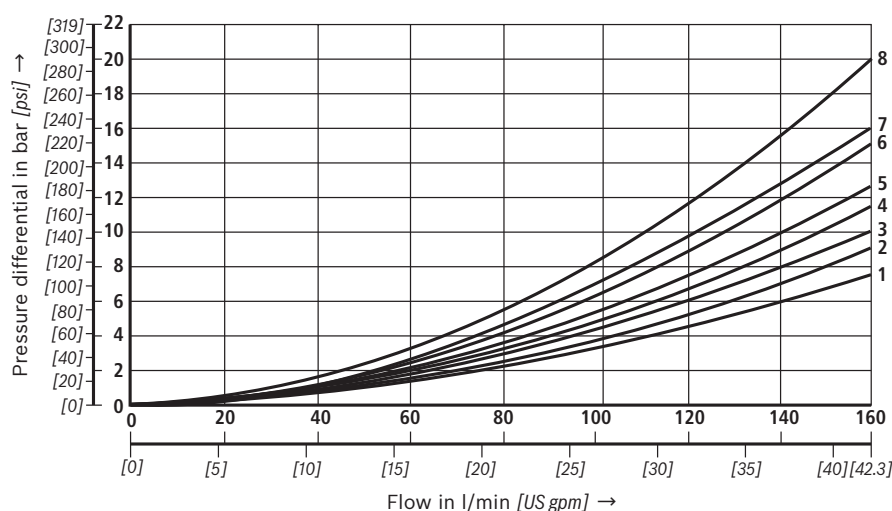
\Delta p - q_v characteristic curves
