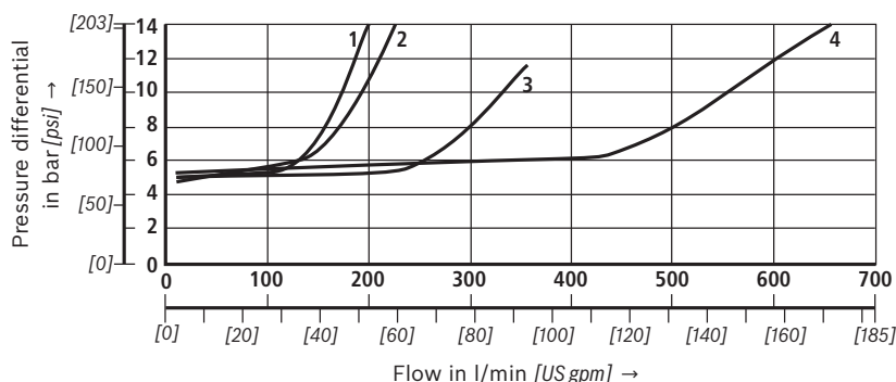
\Delta p - q_v characteristic curve (measured with HLP46, \vartheta_{oil} = 40^\circ \text{C} \pm 5^\circ \text{C} [104°F ± 9°F])
