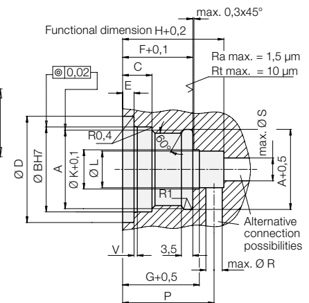
Manifold-mounting hole
