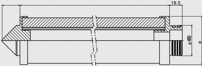
Type 7: Bayonet (2x 226 O-ring), locating spigot 25.5 L1
