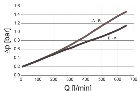
\Delta p optimized DFFX 330, 500, 660, 990, 1320
