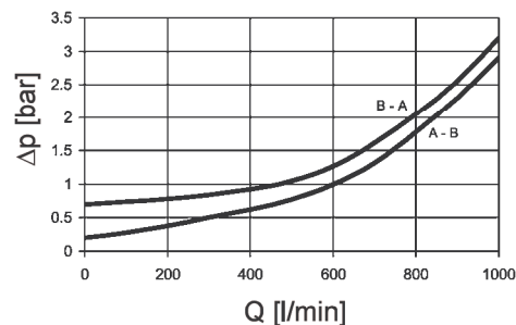
\Delta p optimized DFFX 330, 500, 660, 990, 1320
