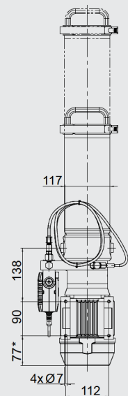
View A
