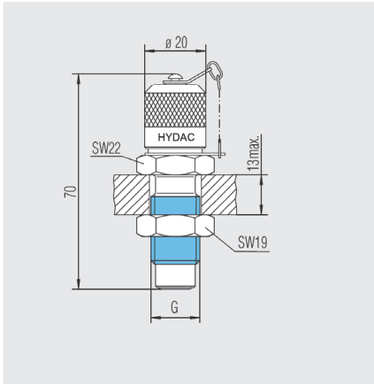
For solderfree screw-in pipe connection acc. to DIN 2353, opposite end: TestPoint 1620 connection (M16 x 2)
