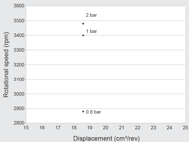
Self-priming capability
