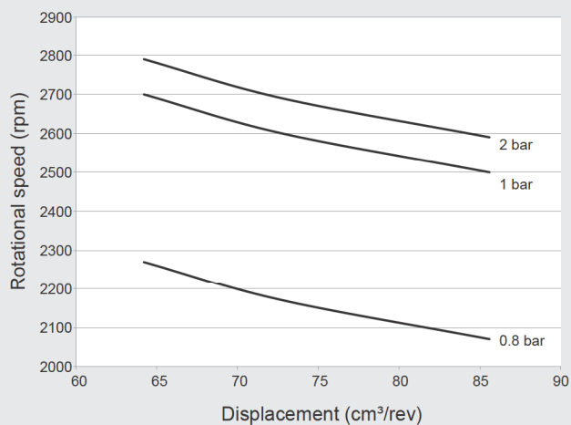
Self-priming capability
