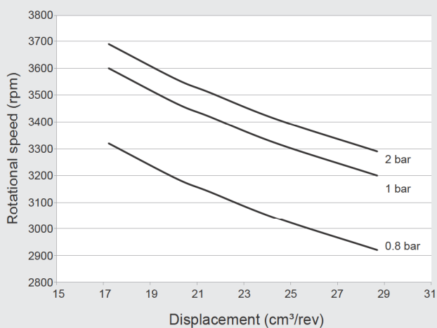
Self-priming capability
