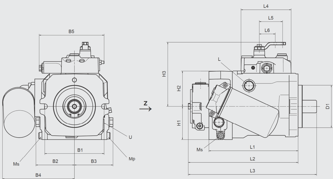
View Z
