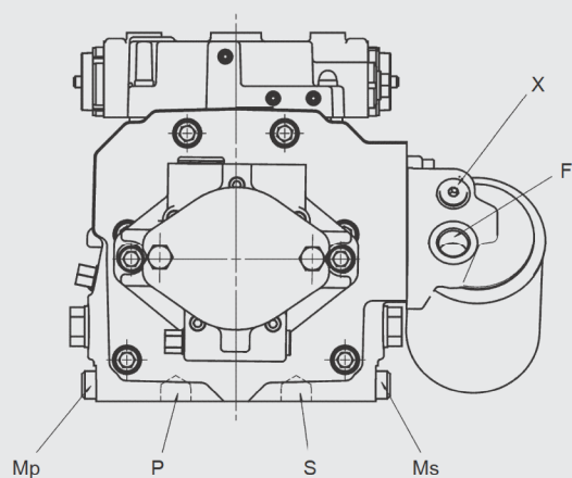
View Z
