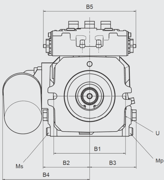
View Z
