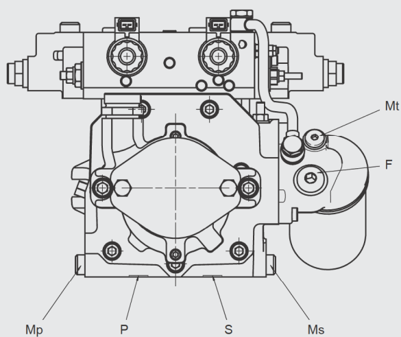
View Z
