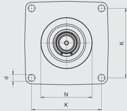
4-hole flange
