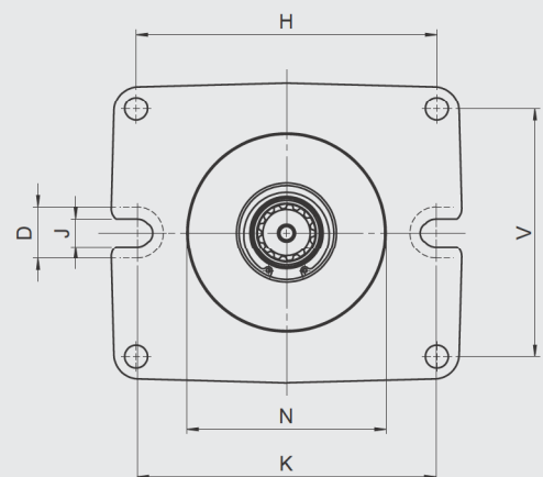
2-hole flange with 4 additional bores
