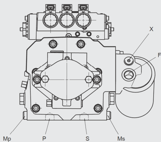
View Z
