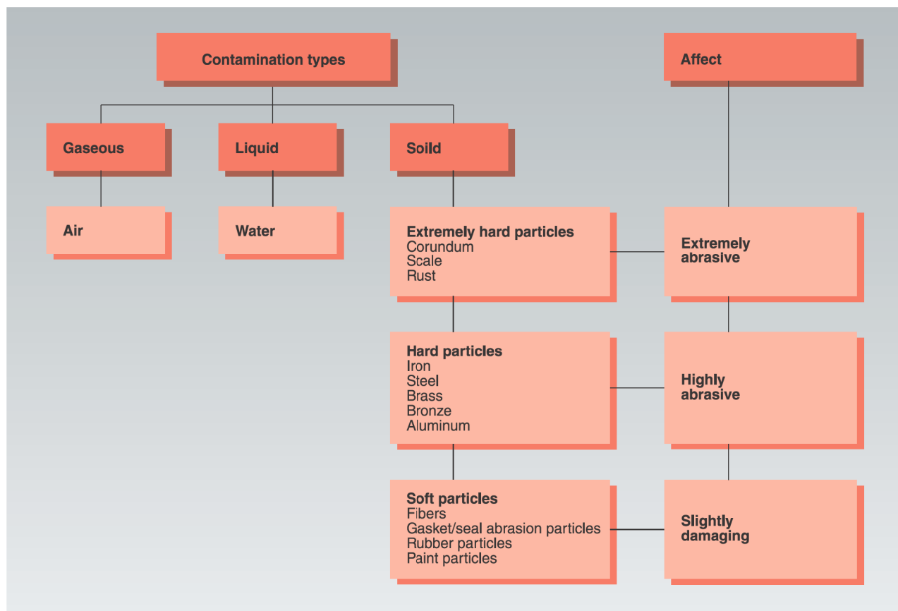
Fig. 1: Contamination Types
