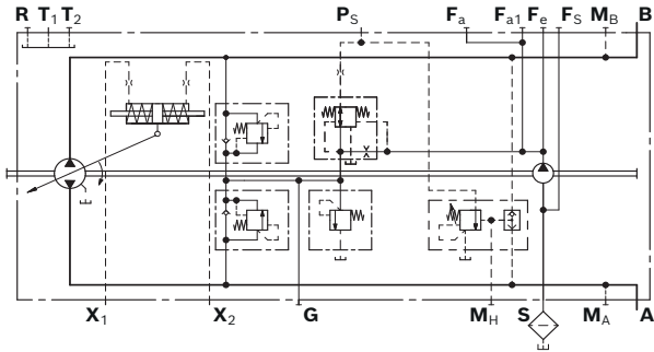
▼ Circuit diagram, version with DA control valve 1)
