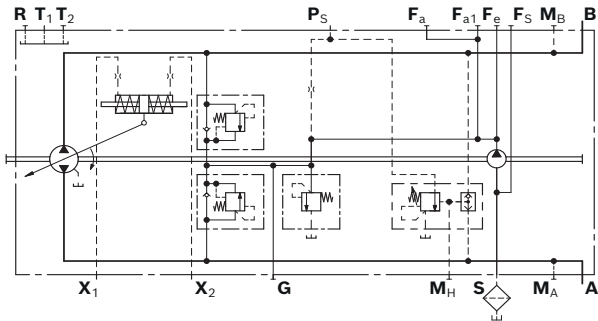
▼ Circuit diagram, version with DA control valve 1)
