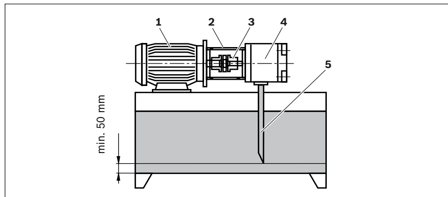
Fig. 4: Recommendation for arrangement of the suction line
