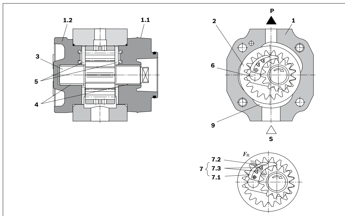
Fig. 2: Layout of the Internal gear pump
