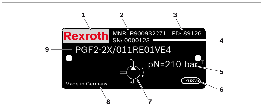
Fig. 3: Name plate Internal gear pump PGF
