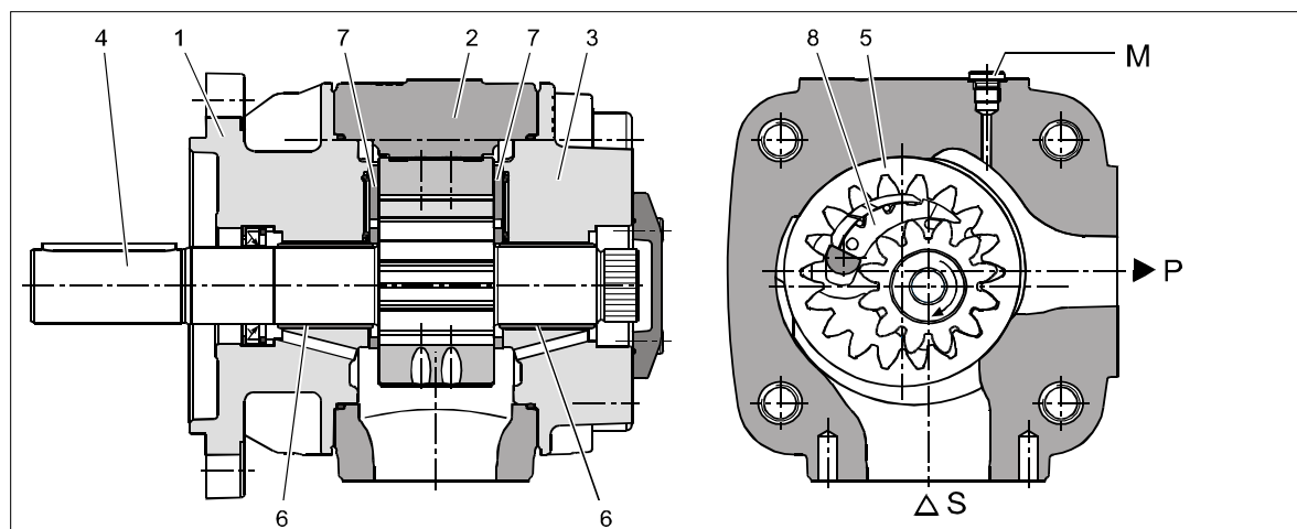
Fig. 2: Set-up of the internal gear pump
