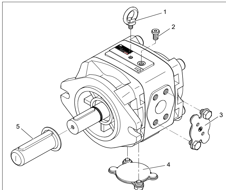
Fig. 1: Scope of delivery internal gear pump PGH.-3X
