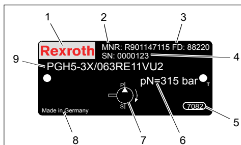
Fig. 3: Example nameplate internal gear pump
