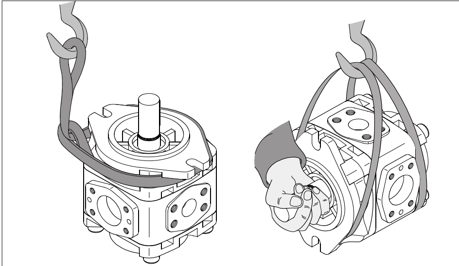
Fig. 5: Mounting using a belt
