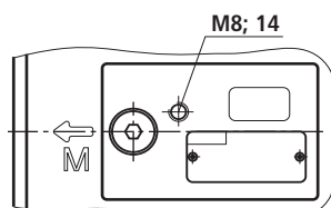
Transport thread PGH4-3X/...
