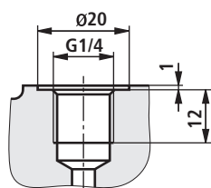
Measuring port PGH4-3X/... and PGH5-3X/...
