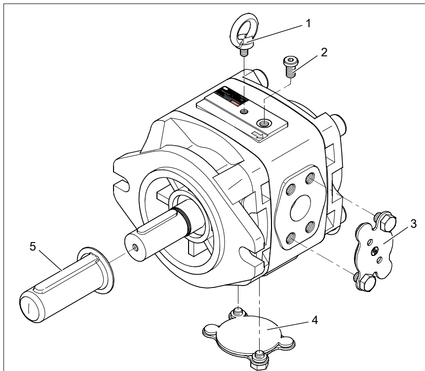
Fig. 1: Scope of delivery internal gear pump PGH.-3X
