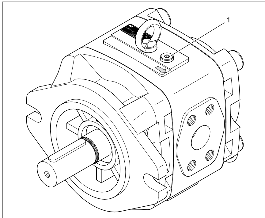
Fig. 9: Bleed and measurement port internal gear pump
