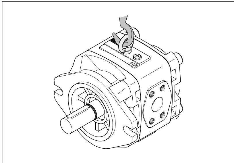
Fig. 4: Mounting using the ring bolt
