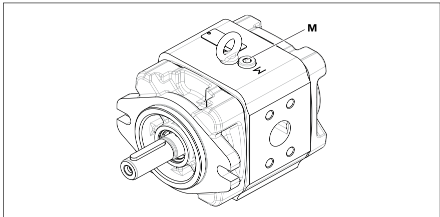
Fig. 9: Bleeding and gauge port (M)
