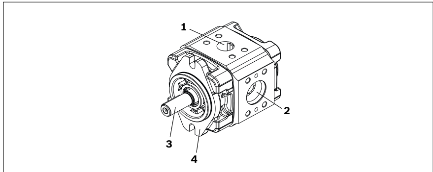
Fig. 8: Internal gear pump installation PGM
