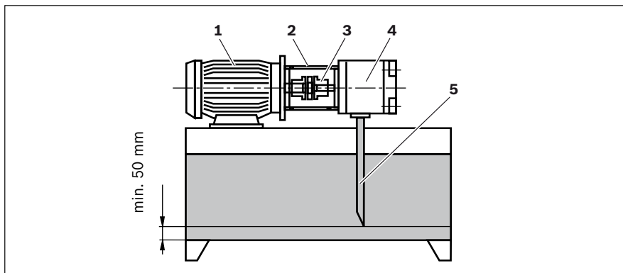
Fig. 6: Recommendation for arrangement of the suction line
