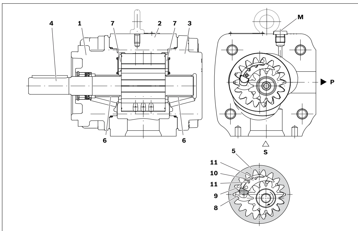
Fig. 2: Assembly of the Internal gear pump
