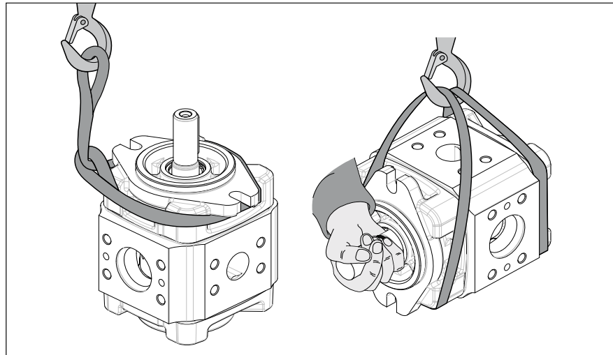
Fig. 5: Transportation with lifting strap
