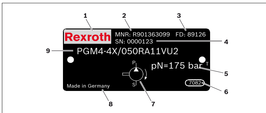
Fig. 3: Name plate Internal gear pump PGM
