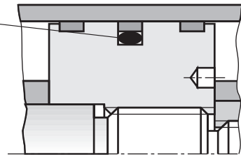
Variant for piston rod Ø 50, 63 and 80 mm
