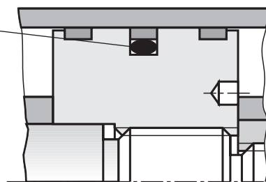
Variant for piston rod Ø 50, 63 and 80 mm
