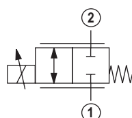
Symbol "N" – normally closed
