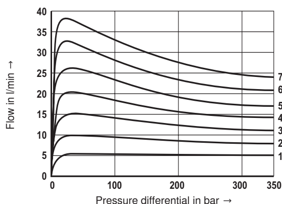
Direction of flow ① → ② Symbol "N"
