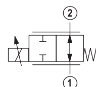
Symbol "P" – normally open
