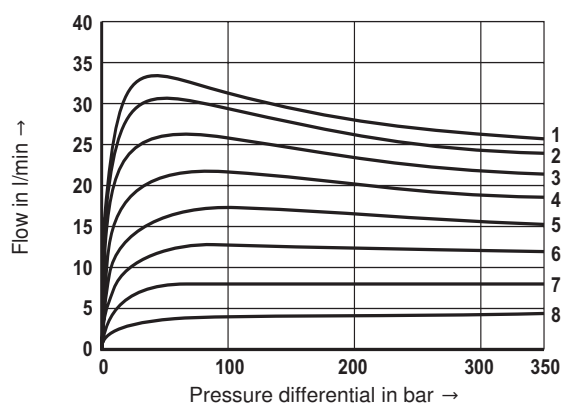
Direction of flow ① → ② Symbol "P"
