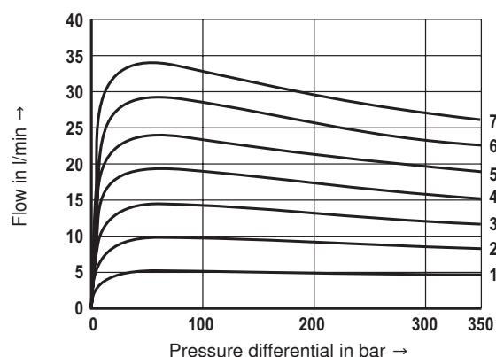
Direction of flow ② → ① Symbol "N"
