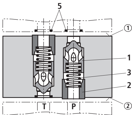
Section 1: Type Z1S 6 F (straight-through valve)
