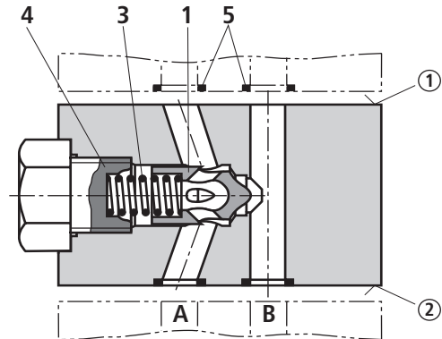
Section 2: Type Z1S 6 BA (angle valve)
