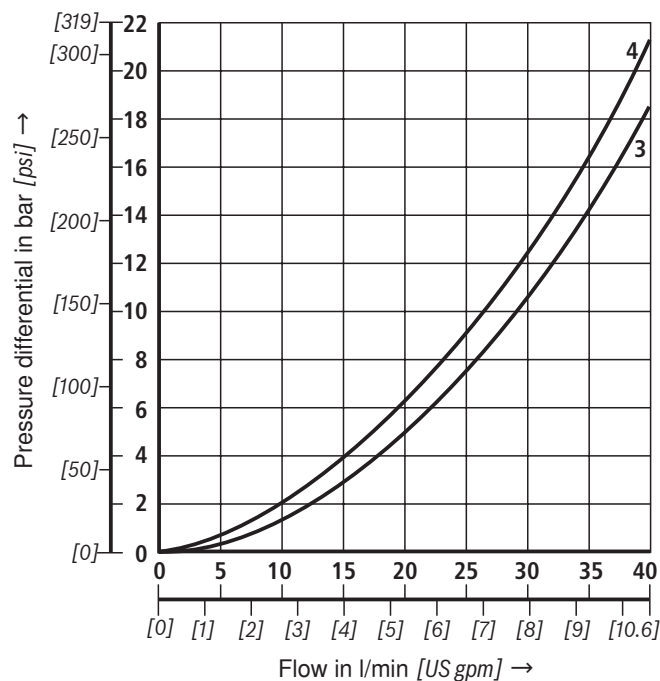
\Delta p - q_v characteristic curves 4/2 directional poppet valve
