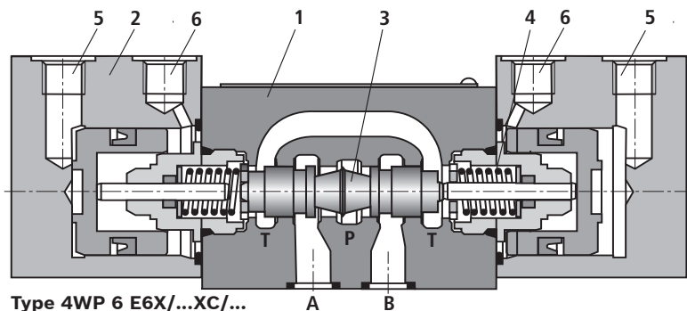
Type 4WP 6 E6X/...XC/...
