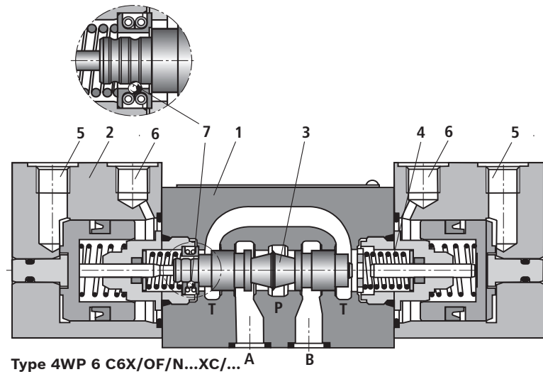
Type 4WP 6 C6X/OF/N...XC/...
