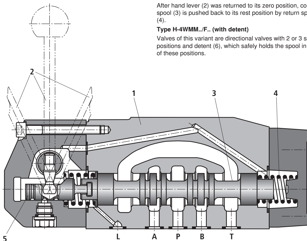
Type H-4WMM 16 E 7X/...
