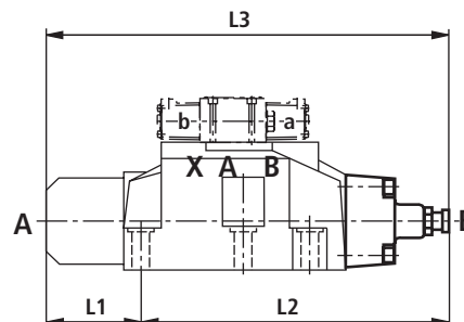
Stroke limitation on side B
