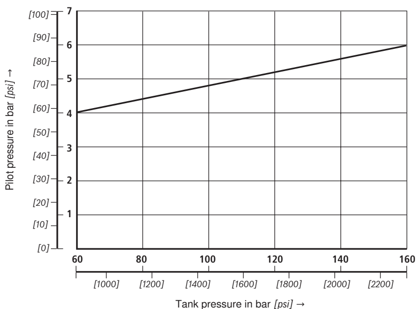
Minimum pilot pressure in dependence upon tank pressure (type WPH)
