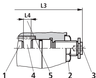
Stroke limitation on side A
