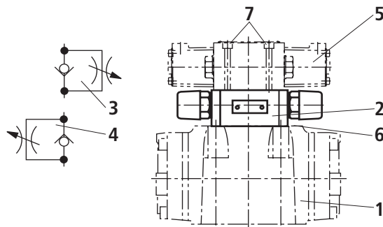
Type 4W.H 10 ..4X/...S
