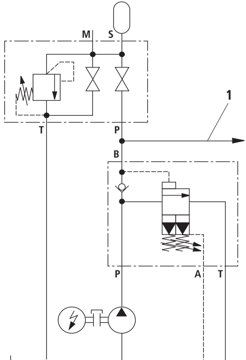
Hydo system with pressure accumulator
