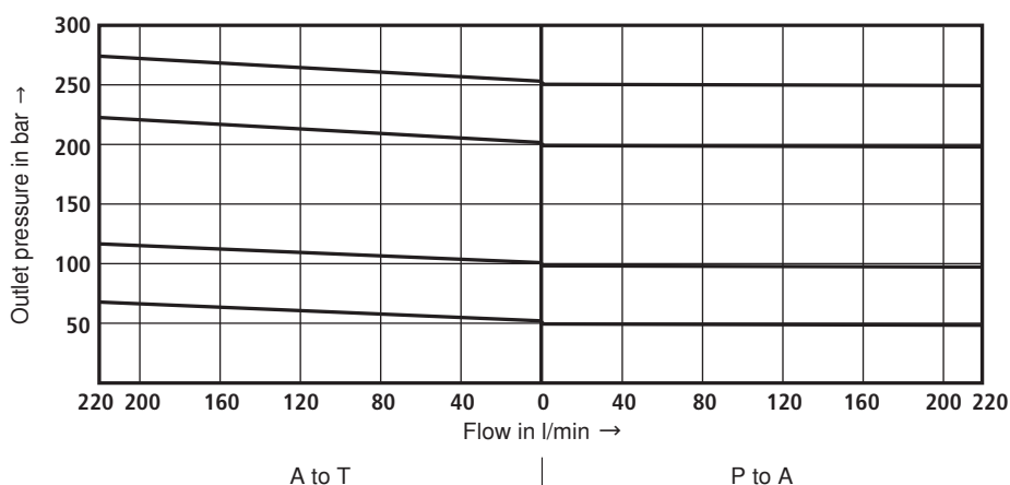
Outlet pressure p_A in dependence on flow q_v
