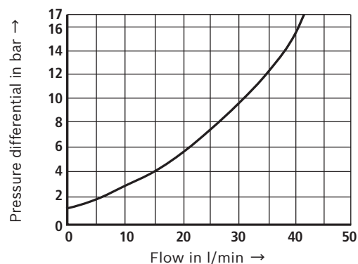
\Delta p - q_v characteristic curve via check valve B \rightarrow A; orifice closed
