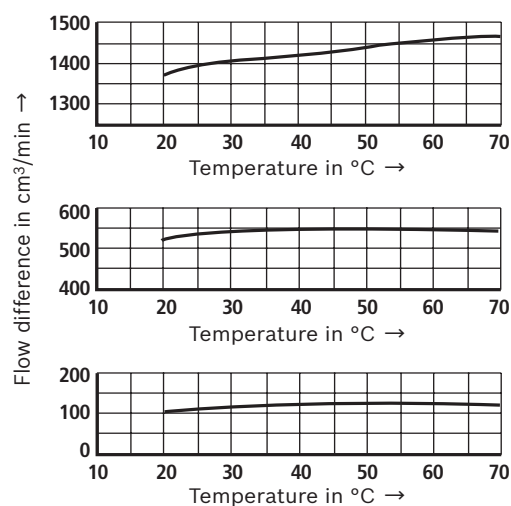
Temperature dependency at \Delta p = 20 \text{ bar}
