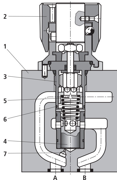
Type 2FRM 6 B76-3X/.M...
