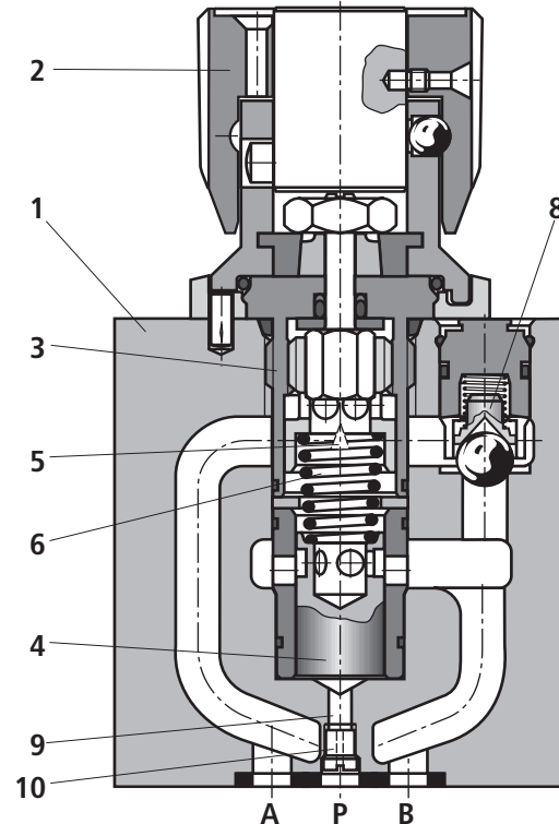
Type 2FRM 6 A76-3X/..RV
