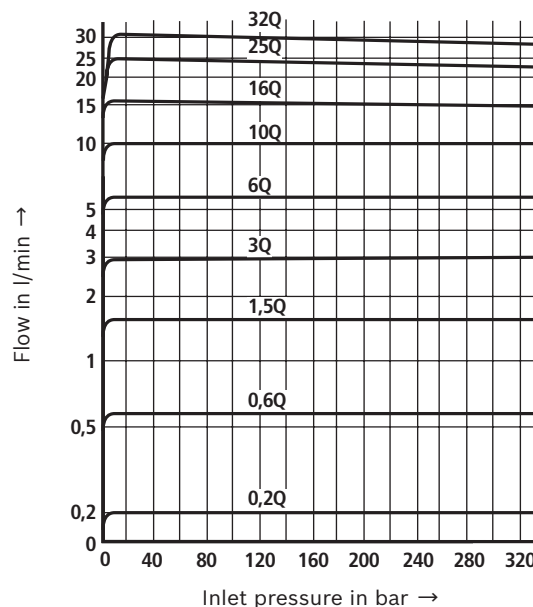
p_E - q_v characteristic curve
