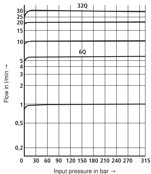
Flow q_v against the input pressure p_E
