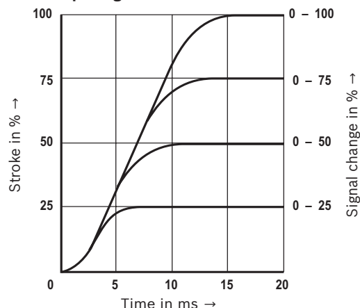
Transition function with stepped electric input signals
