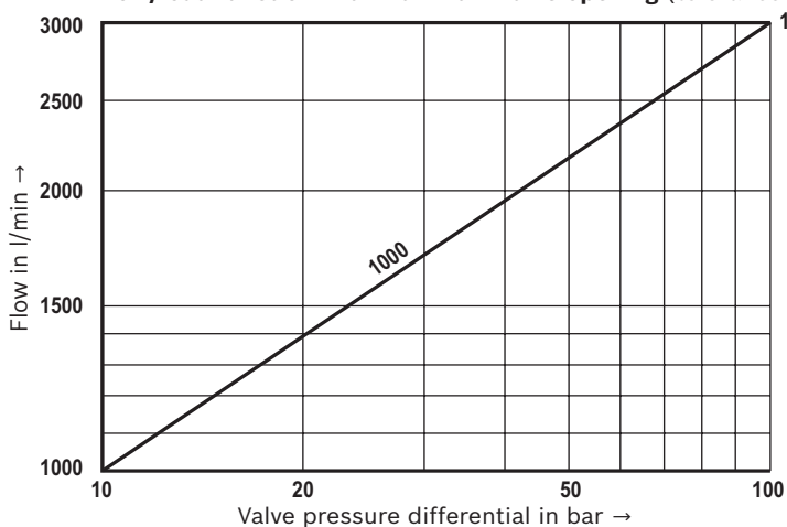
Flow/load function with maximum valve opening (tolerance \pm 10\% )
