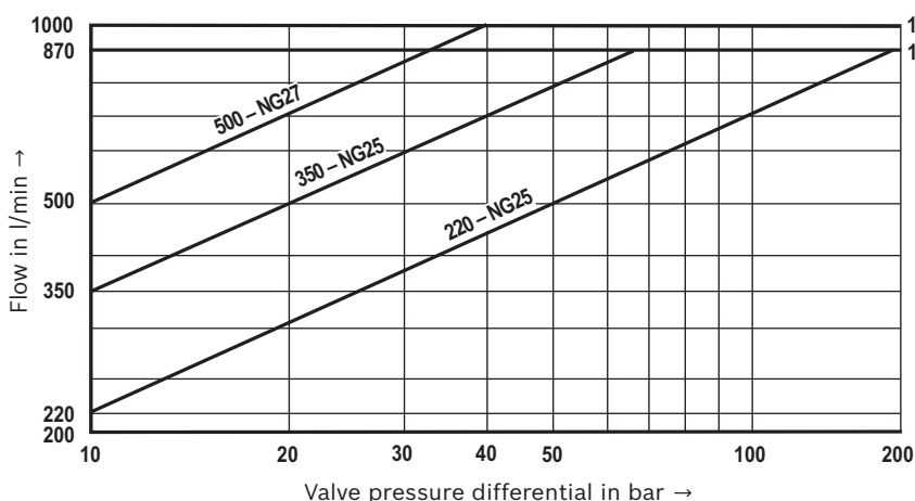
Flow/load function with maximum valve opening (tolerance ±10%)
