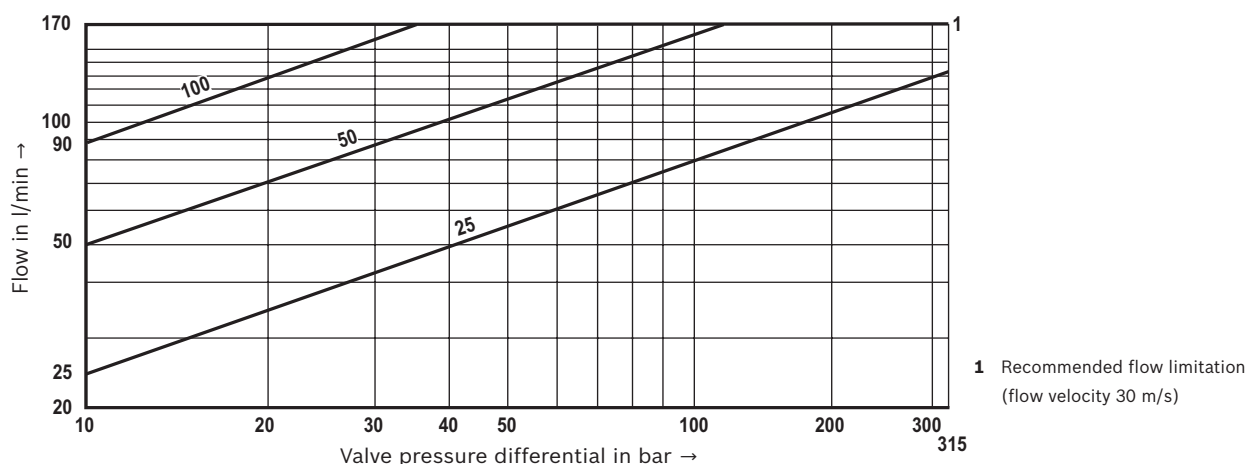
Flow/load function with maximum valve opening (tolerance ±10%)
