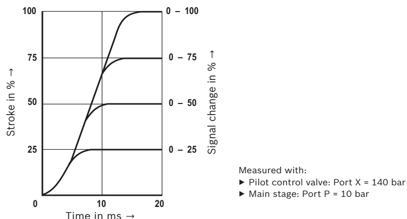
Transition function with stepped electric input signals
