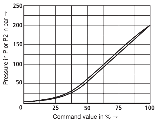
Pressure rating 200 bar (with VT-SSPA1) plug-in amplifier
