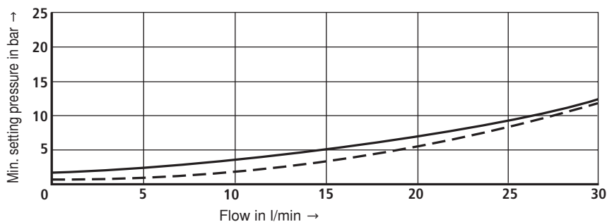
Pressure rating 50 bar
