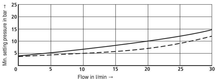
Pressure rating 100 bar
