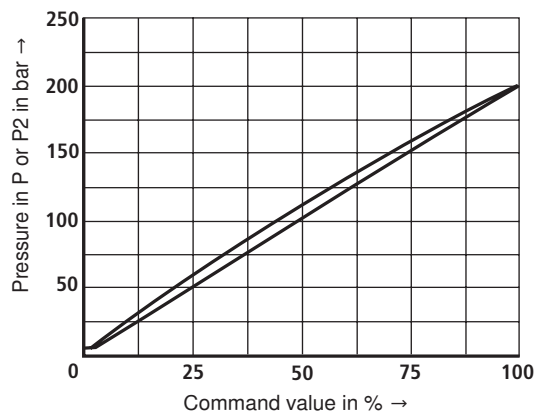
Pressure rating 200 bar ("y" external and internal)
