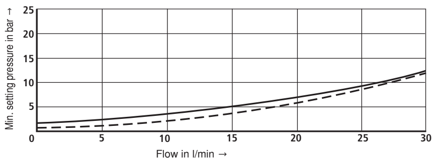
Pressure rating 25 bar
