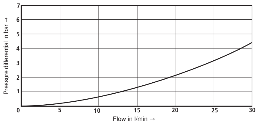
Pressure differential A1 → A2 and B1 → B2
