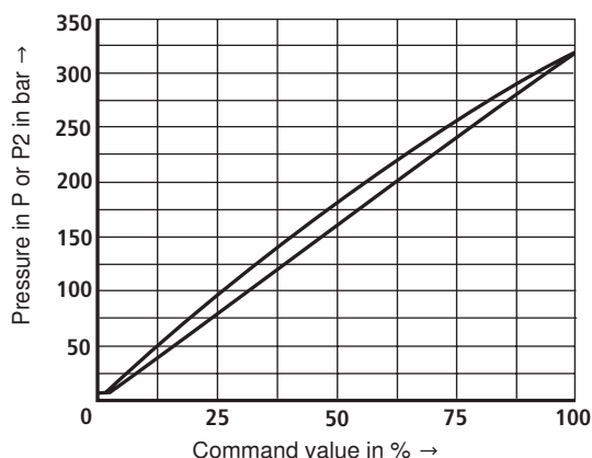
Pressure rating 315 bar ("y" external and internal)
