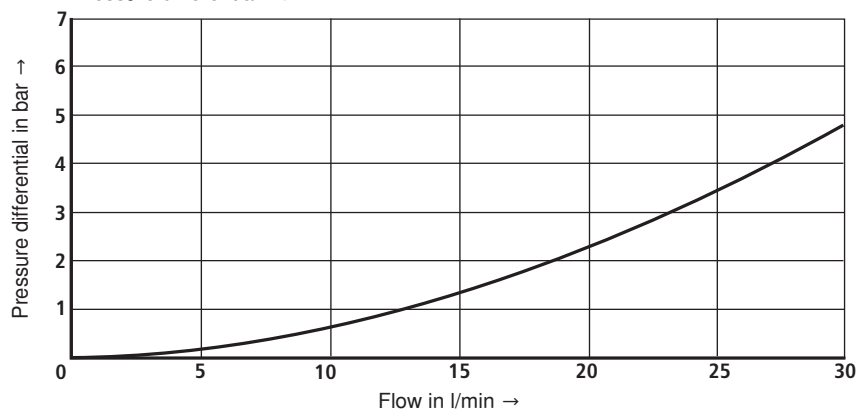
Pressure differential P1 → P2
