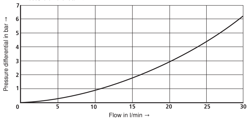
Pressure differential T1 → T2
