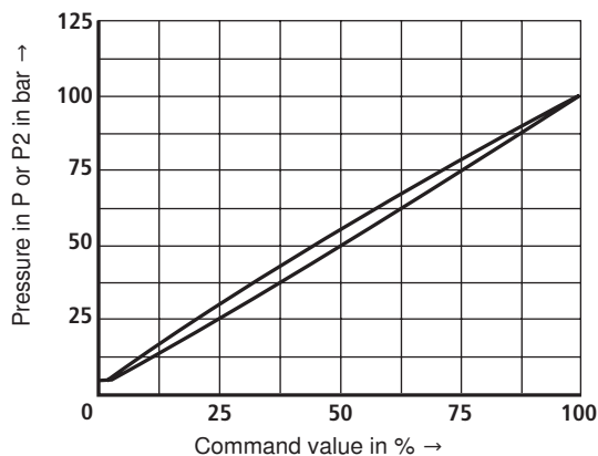
Pressure rating 100 bar ("y" external and internal)
