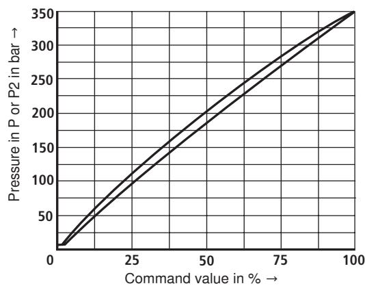
Pressure rating 350 bar ("y" external and internal)
