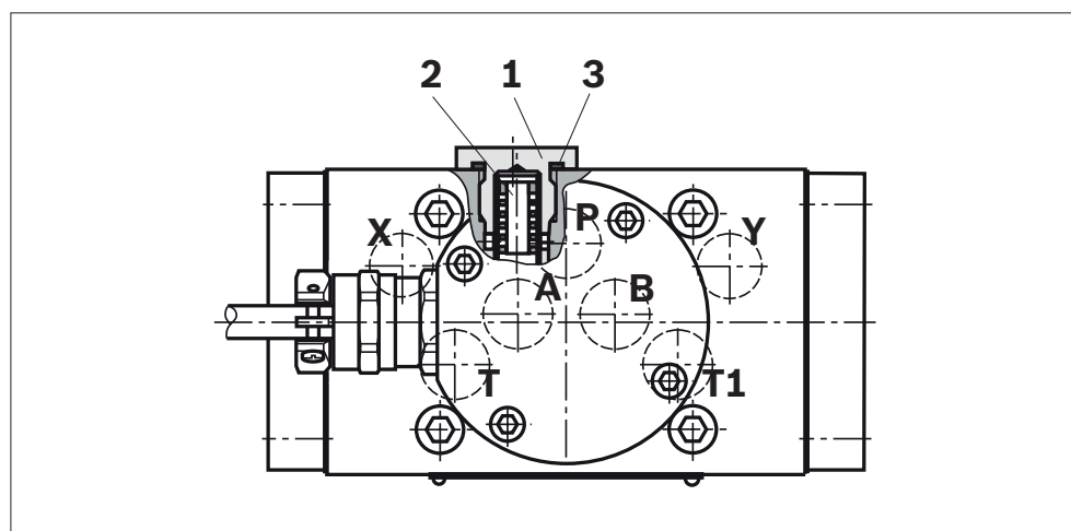
Fig. 2: Filter element
