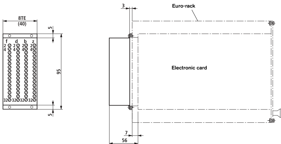
Adapter, 64-pin, form G
