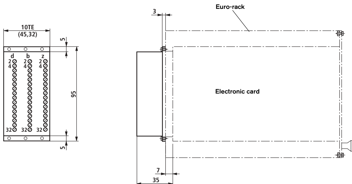
Adapter, 48-pin, form F
