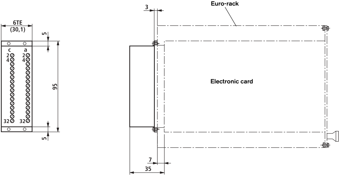
Adapter, 32-pin, form D
