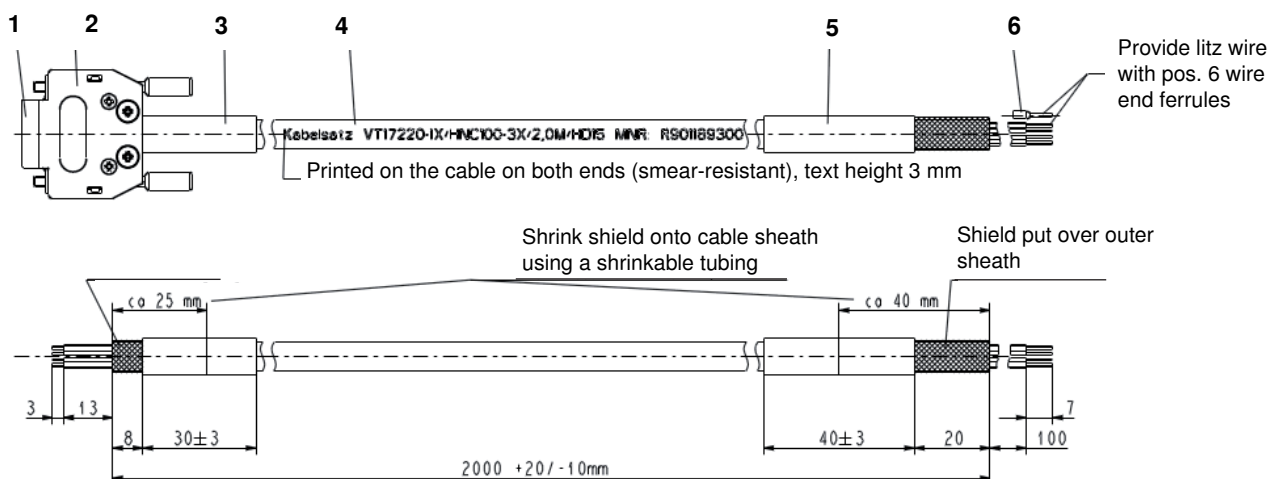
Fig. 6: Wiring diagram for analog or digital interface
