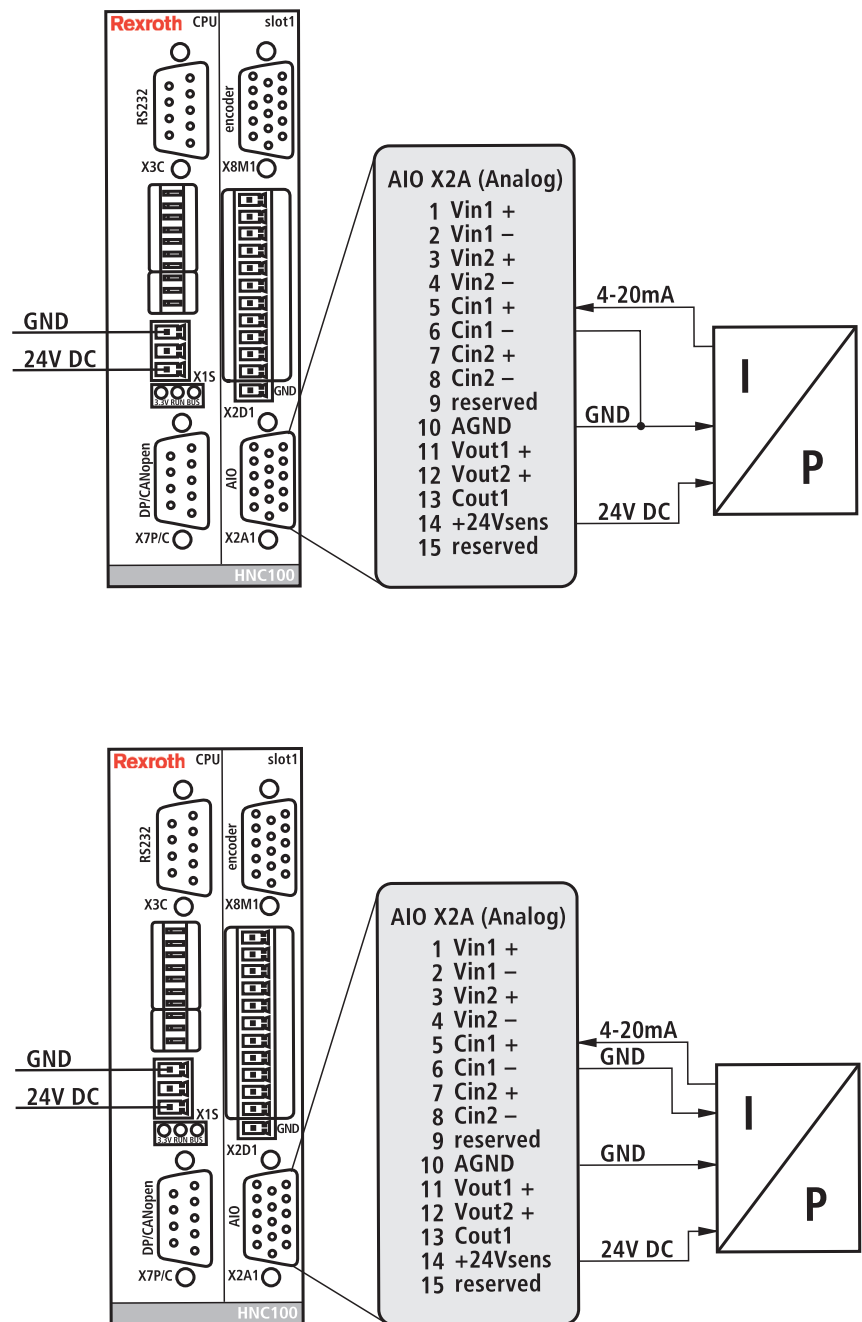
Fig. 7: Wiring for pressure transducers
