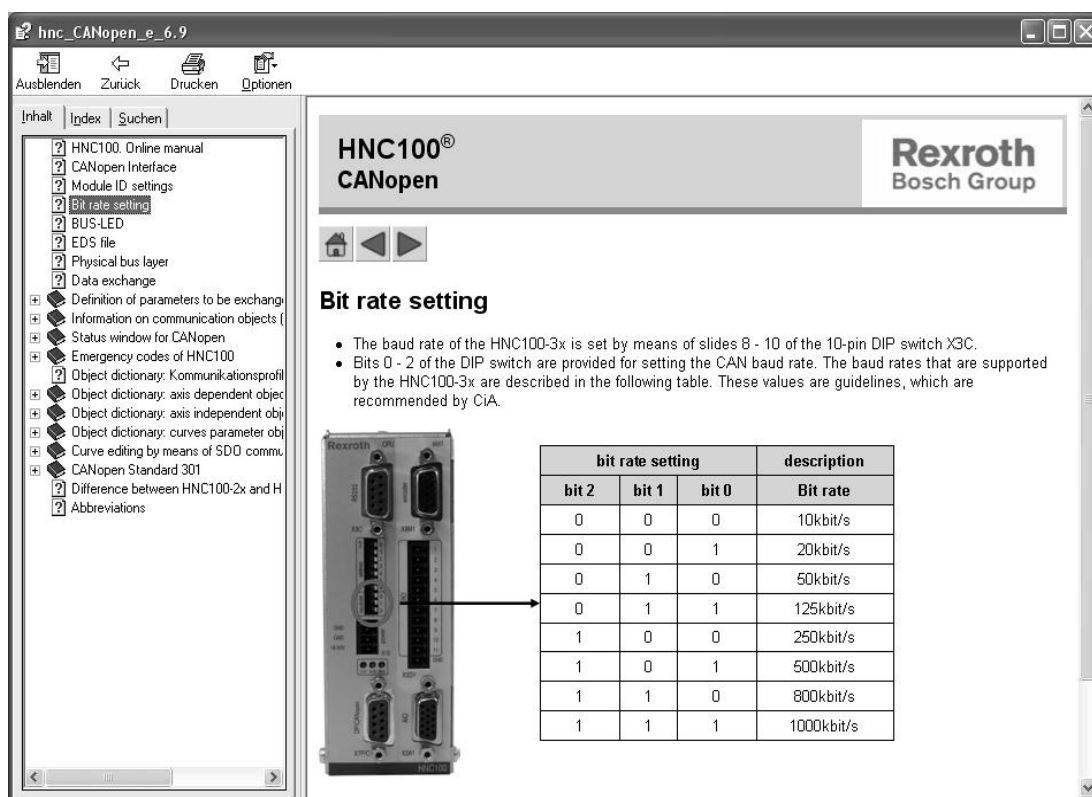
Fig. 11: Baud rate for CANopen
