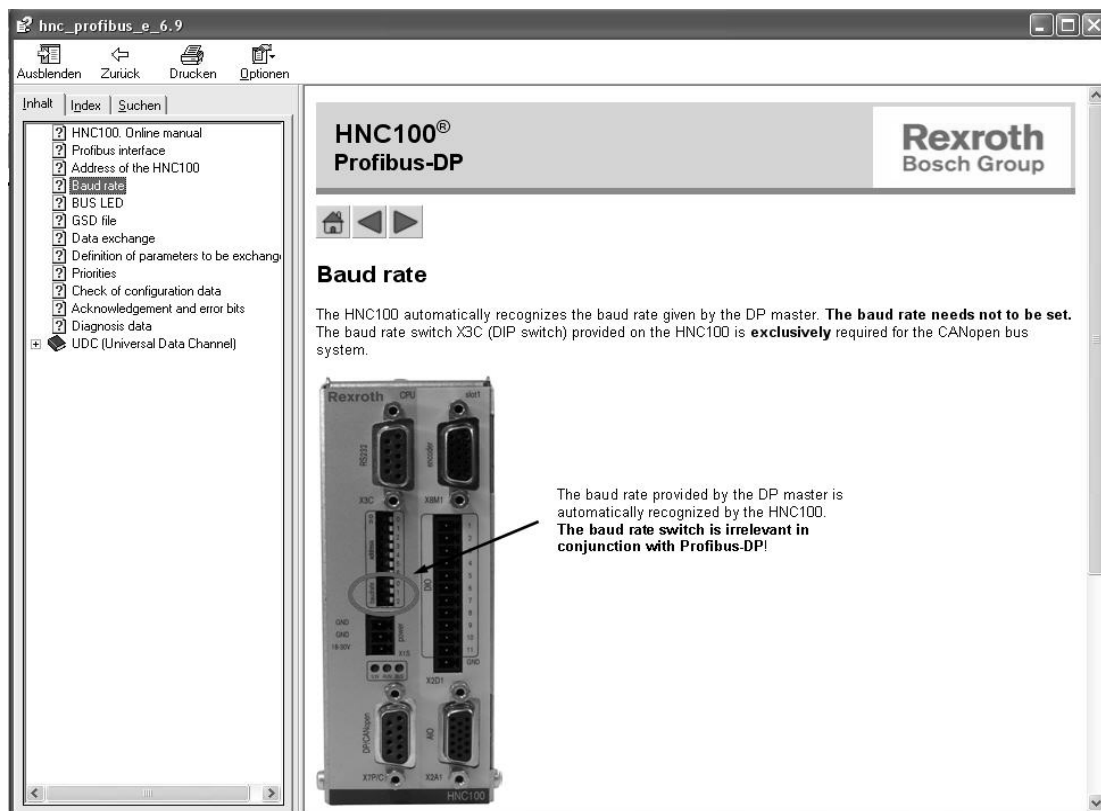
Fig. 14: PROFIBUS DP baud rate
