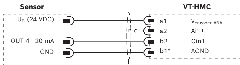
Fig. 9: Sensor supplied by VT-HMC...1X (3-conductor)
