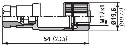
Cable socket for plug K24
