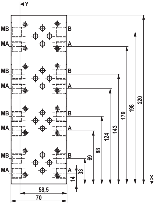
Dimensions Dimension Z = 64 mm
