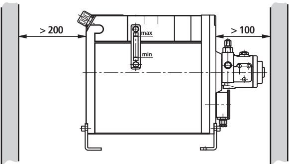
Necessary minimum distance to the wall for perfect cooling.
