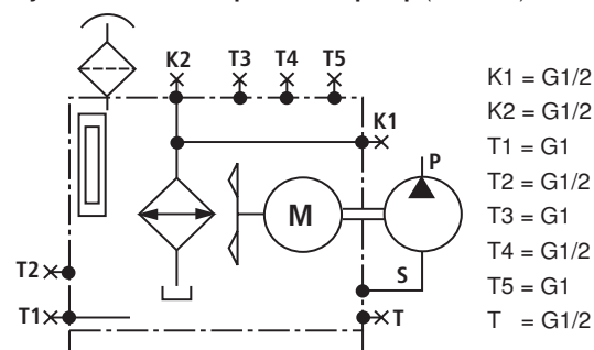
Symbol for fixed displacement pump (GF2, AZ)
