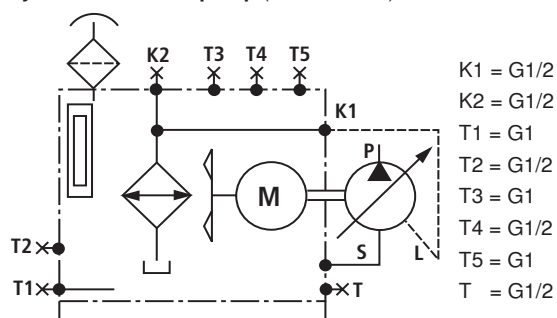
Symbol for control pump (A10VSO, V7)
