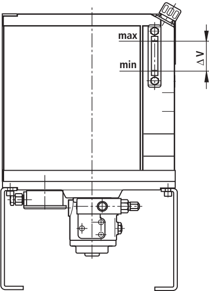
Installation variant: Vertical mounting
