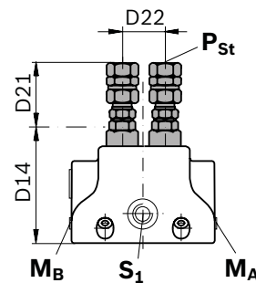
Detailed view Z: Version with pressure boost facility (code 192)
