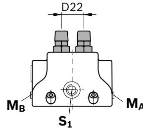
Detailed view Z: Version without pressure boost facility (code 191)
