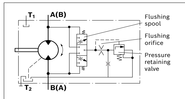
Circuit diagram
