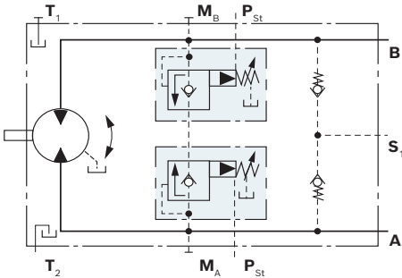
▼ Circuit diagram version with pressure sequencing stage 09S
