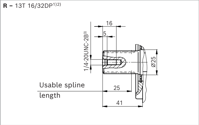
Connection table A10FZG
