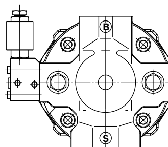
View Y with clockwise rotation
