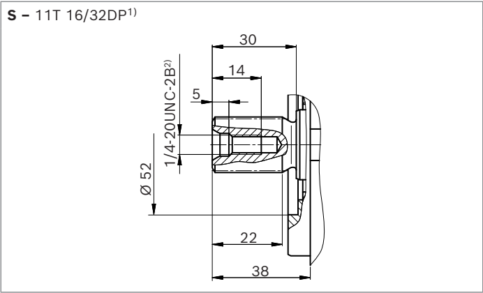
Connection table A10VZG
