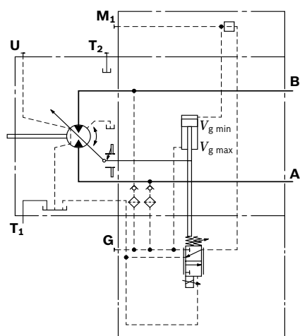
▼ Circuit diagram EP1, EP2 size 280 (positive control)
