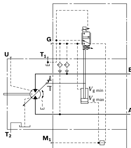
▼ Circuit diagram EP5, EP6 size 60 to 215 (negative control)
