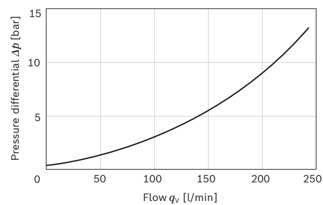
▼ Boost characteristic NG55, NG80 and NG107
