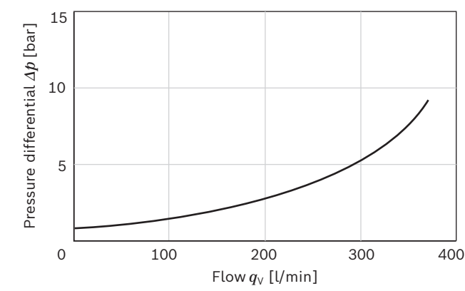
▼ Boost characteristic NG160
