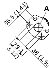
Detail Z
