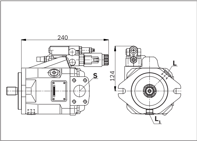
▼ ED7. / ER7. – Electro-proportional pressure control, series 52
