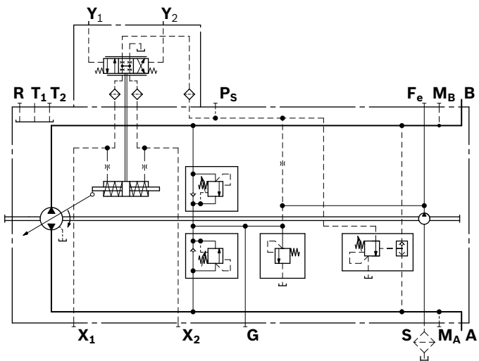
▼ Circuit diagram, version with pressure cut-off
