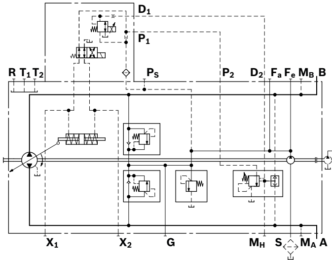
▼ Circuit diagram, standard version ED2
