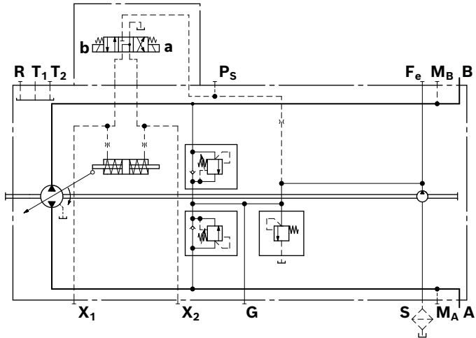
▼ Circuit diagram, version without pressure cut-off
