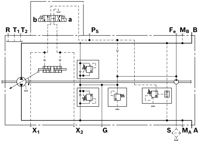
▼ Circuit diagram, version with pressure cut-off
