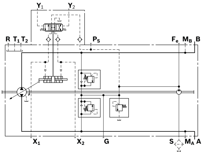
▼ Circuit diagram, version without pressure cut-off
